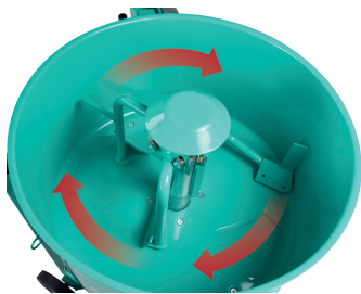
The rotation direction of the paddles allows to disintegrate any lumps and resume normal mixing without direct manual intervention.
